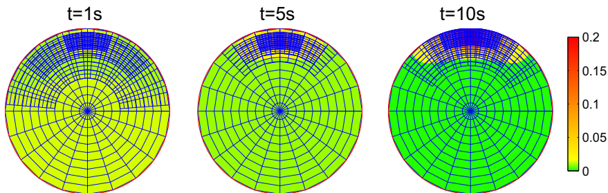
Fig. 2. Contour plots for concentration of AB in the system (30) calculated using cIIF2 with AMR. The parameters for the simulation are D = 1 \mu\text{m}^2 \text{s}^{-1} , k_{on} = 0.1 (\mu\text{M s})^{-1} , k_{off} = 0.3 \text{s}^{-1} , j_{on} = 1 (\mu\text{M s})^{-1} , j_{off} = 0.005 \text{s}^{-1} , j_{con} = 0.1 (\mu\text{M s})^{-1} .
